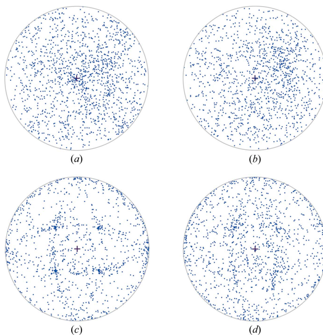
Figure 4 Stereographic projections illustrating the crystal orientation of 1000 randomly selected crystals for each loading method and crystal type: (a) pipette-loaded AcNiR, (b) PolyPico-loaded AcNiR, (c) pipette-loaded HEWL and (d) PolyPico-loaded HEWL. The plots represent the direction of the 001 hkl of each crystal (reindexed in P1 ) relative to the beam direction ( z ) which is shown as the central '+' into the page. A point at 12 o'clock on the circular projection represents a 90^\circ rotation of the crystal around x whereas the point at 3 o'clock represents a 90^\circ rotation around y . Plots were produced using the module dials.stereographic_projection (Winter et al. , 2018).
