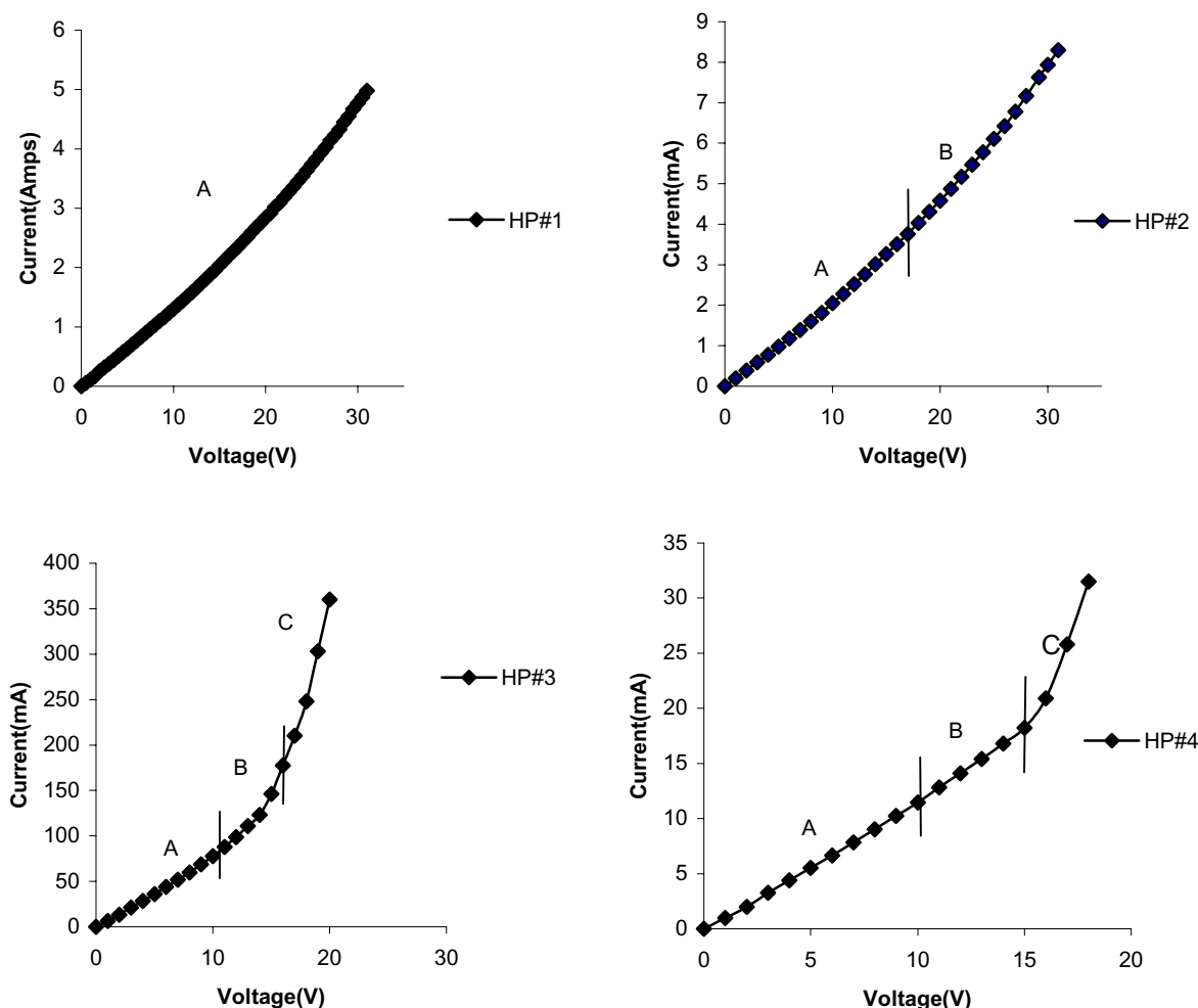
Figure 8. I-V plots for the \text{In}_2\text{O}_3/\text{SiO} samples produced at high pressure.
