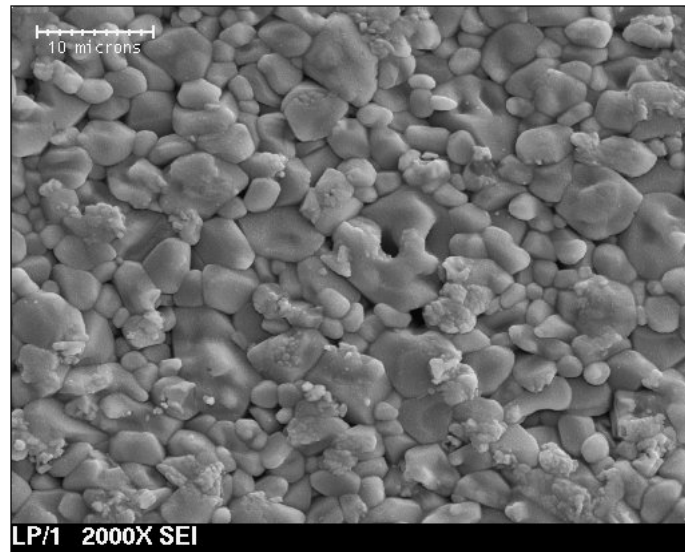
Figure 1. SEM image of the surface of the In 2 O 3 /SiO thin films obtained at a magnification of 2,000.
