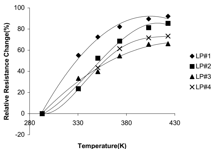
Figure 9. The relative resistance change expressed as a percentage against increasing temperature for the \text{In}_2\text{O}_3/\text{SiO} samples produced at low pressure.
