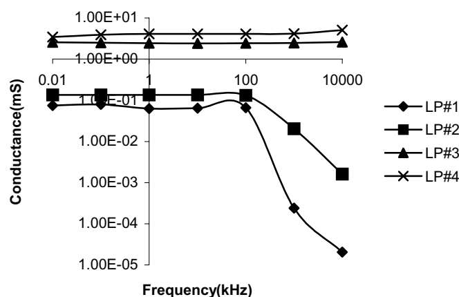
Figure 3. The variation of conductance against frequency for the In 2 O 3 /SiO samples produced at low vacuum pressure.
