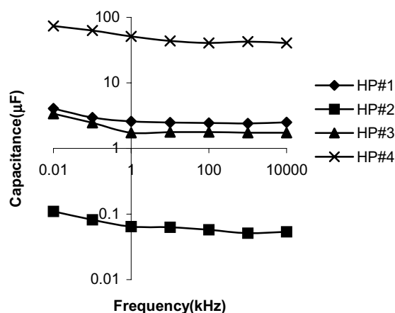
Figure 6. The variation of capacitance against frequency for the \text{In}_2\text{O}_3/\text{SiO} samples produced at high vacuum pressure.
