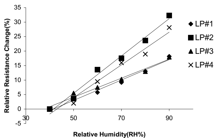
Figure 12. Humidity Sensitivity Curves for In 2 O 3 /SiO at 60°C.
