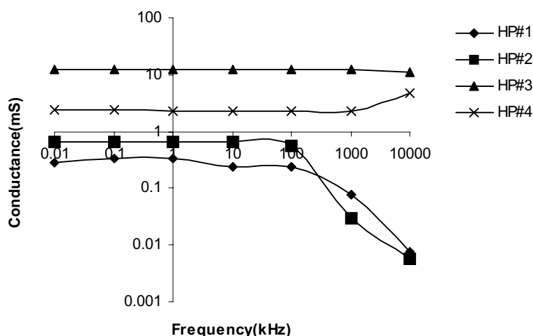
Figure 4. The variation of conductance against frequency for the \text{In}_2\text{O}_3/\text{SiO} samples produced at high vacuum pressure.
