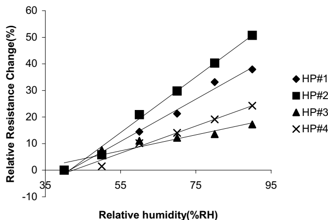
Figure 13. Humidity Sensitivity Curves for In 2 O 3 /SiO, produced at high vacuum pressure, at 30°C.
