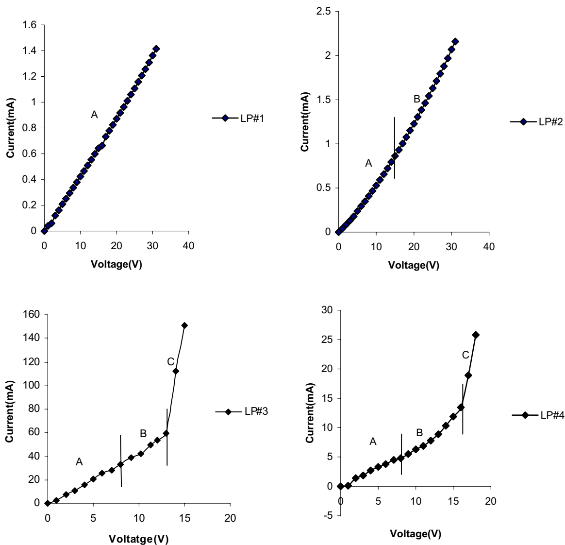
Figure 7. I-V plots for the \text{In}_2\text{O}_3/\text{SiO} samples produced at low pressure.
