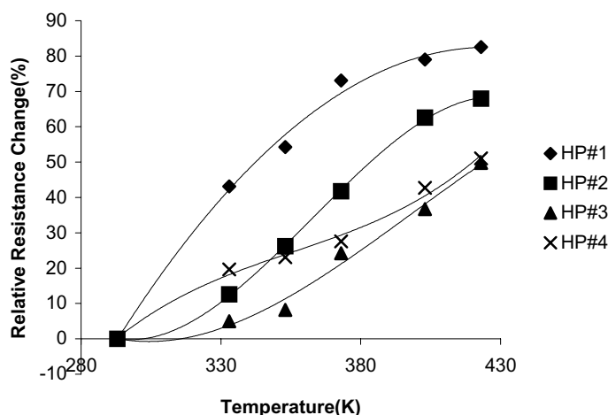
Figure 10. The relative resistance change expressed as a percentage against increasing temperature for the In 2 O 3 /SiO samples produced at high pressure.
