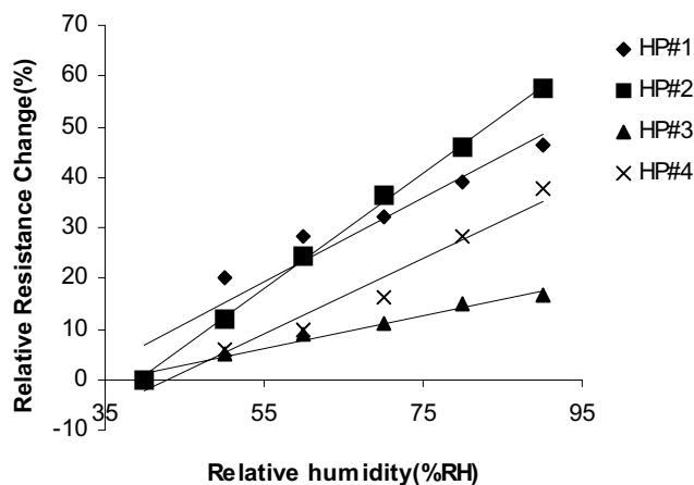
Figure 14. Humidity Sensitivity Curves for In 2 O 3 /SiO, produced at high vacuum pressure, at 60°C.
