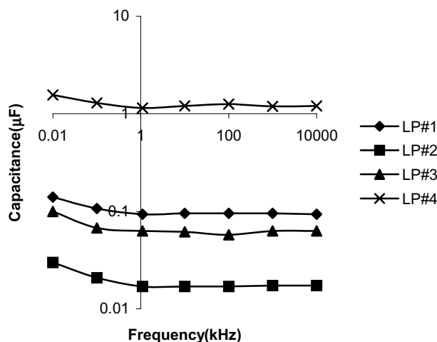
Figure 5. The variation of capacitance against frequency for the \text{In}_2\text{O}_3/\text{SiO} samples produced at low vacuum pressure.
