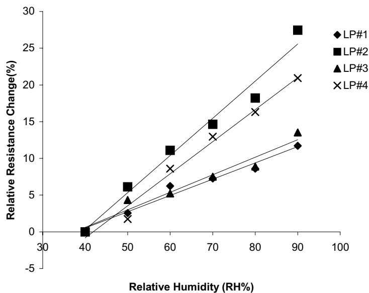
Figure 11. Humidity Sensitivity Curves for In 2 O 3 /SiO at 30°C.
