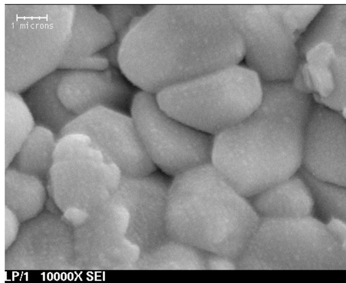
Figure 2. SEM Image of the surface of the In 2 O 3 /SiO thin films obtained at a magnification of 10,000.
