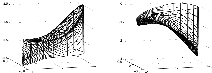
FIGURE 1. Multiple boundary-layer solutions of model problem (5.1); in the interior subdomain u(x) \approx z(x) (left) or u(x) \approx -z(x) (right), where \pm z(x) are stable solutions of the reduced problem (1.4).
