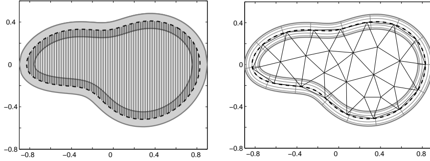
FIGURE 2. Overlapping boundary-layer subdomain \Omega_{[0,2\sigma]} and interior subdomain \Omega_\sigma (left); layer-adapted tensor-product mesh in \Omega_{[0,2\sigma]} and quasiuniform Delaunay triangulation in \Omega_\sigma (right).
