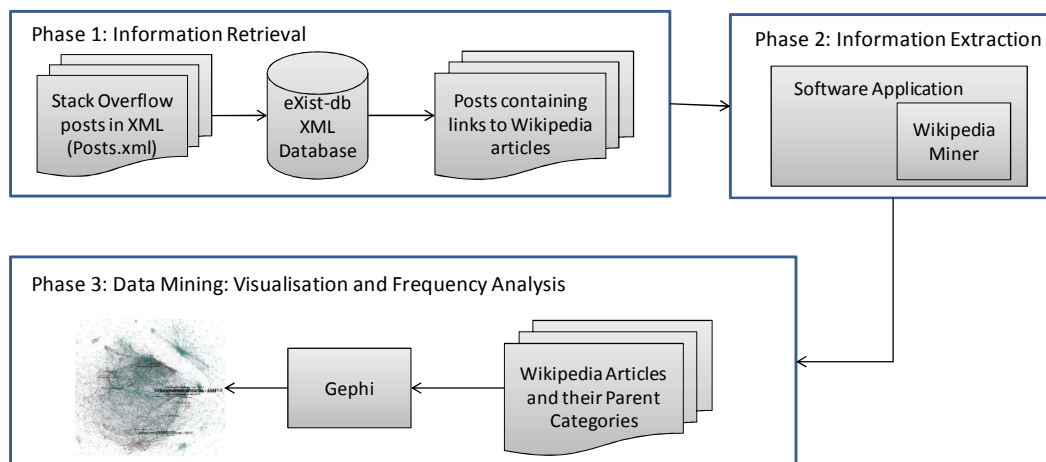
Figure 1: Overview of text mining approach
