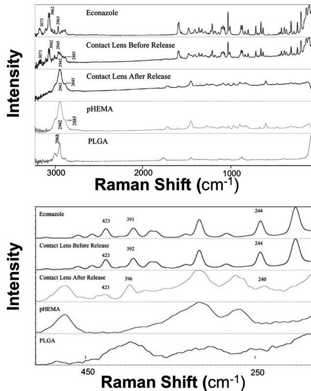
FIGURE 5. Raman spectra of econazole, a pHEMA film, a PLGA film, and a contact lens containing an econazole-PLGA film (PLGA16) before and after 10 days of drug release. Top : shift from 0 to 3300 \text{ cm}^{-1} . Zoom of the Raman spectra ( bottom , 180\text{--}550 \text{ cm}^{-1} ) demonstrated multiple peaks ( 423, 391, \text{ and } 244 \text{ cm}^{-1} ) in the contact lens that were indicative of econazole.
