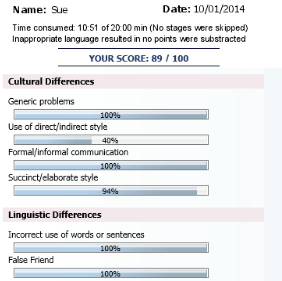
Figure 3. Automatic assessment.
