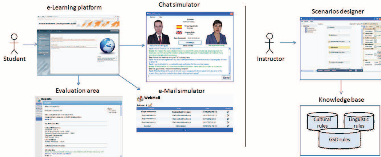
Figure 1. VENTURE's environment.
