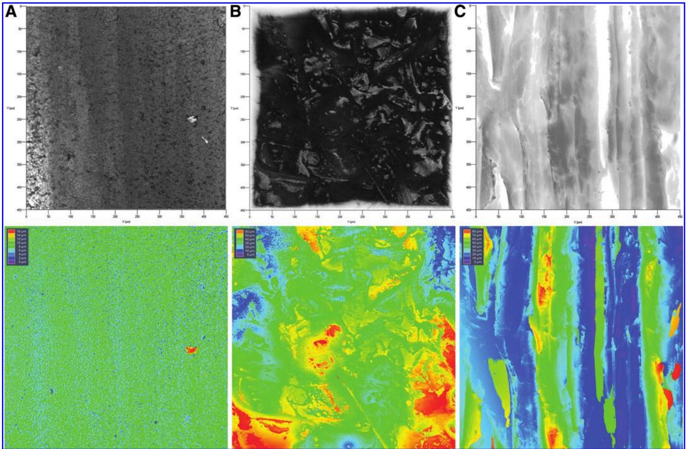
Figure 3. 3D topography and height maps are shown in the top and bottom rows, respectively, for selected phantom materials. Shown are (A) Sylgard 160, (B) TangoPlus FLX930, and (C) HeartPrint Flex. Note the residual machining marks in the case of Sylgard 160, typical of all models produced by the lost-wax casting process. Color images available online at www.liebertpub.com/3DP
