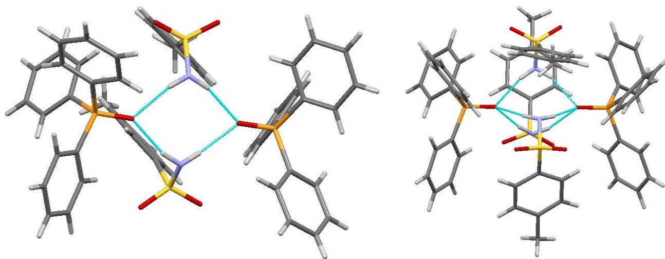
Figure 2 The cococrystals of TSA with PPh 3 O: (i) the 1:1 cococrystal, left, showing the R 4 2 (8) ring and (ii) the 3:2 cococrystal, 17 right, which also has the R 4 2 (8) motif.
