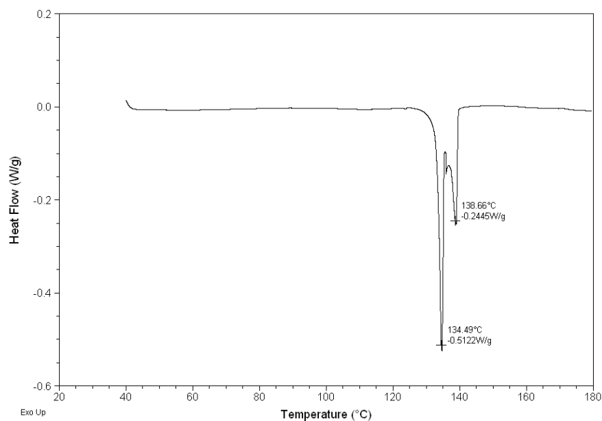
Figure 1: DSC trace of the product obtained from 30 minute grinding of a 1:1 molar mixture of TSA and Ph 3 PO.
