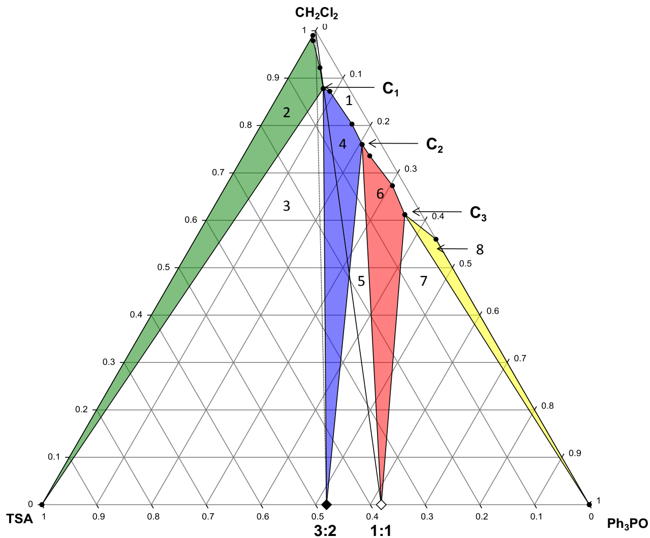
Figure 5: Ternary Phase Diagram for the TSA – Ph 3 PO – CH 2 Cl 2 system at 20 °C. Regions in the diagram are as follows: (1) solution phase; all other regions consist of a saturated solution in contact with (2) TSA only, (3) TSA + 3:2 cocrystal, (4) 3:2 cocrystal only, (5) 3:2 cocrystal + 1:1 cocrystal, (6) 1:1 cocrystal only, (7) 1:1 cocrystal + Ph 3 PO, and, (8) Ph 3 PO only. Values are in mass fraction, total mass basis.
