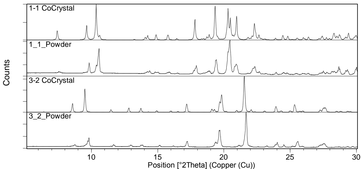
Figure 3: Diffraction patterns of the 1:1 and 3:2 cococrystal as generated from the corresponding CIF for each cococrystal using X'Pert Highscore 2.0 (1-1 CoCrystal, and 3-2 CoCrystal respectively), and PXRD
