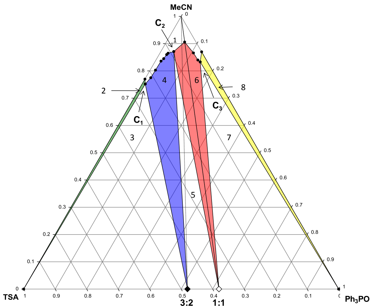
Figure 4: Ternary Phase Diagram for the TSA – Ph 3 PO – MeCN system at 20 °C. Regions in the diagram are as follows: (1) solution phase; all other regions consist of a saturated solution in contact with (2) TSA only, (3) TSA + 3:2 cocrystal, (4) 3:2 cocrystal only, (5) 3:2 cocrystal + 1:1 cocrystal, (6) 1:1 cocrystal only, (7) 1:1 cocrystal + Ph 3 PO, and, (8) Ph 3 PO only. Values are in mass fractions.
