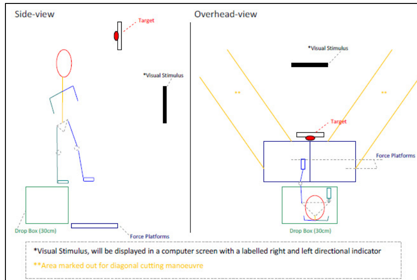
Figure 1. Dynamic Task Set Up
