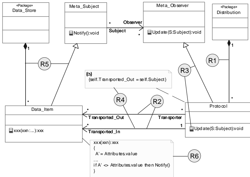
Fig. 2. Observer pattern in a meta-model
