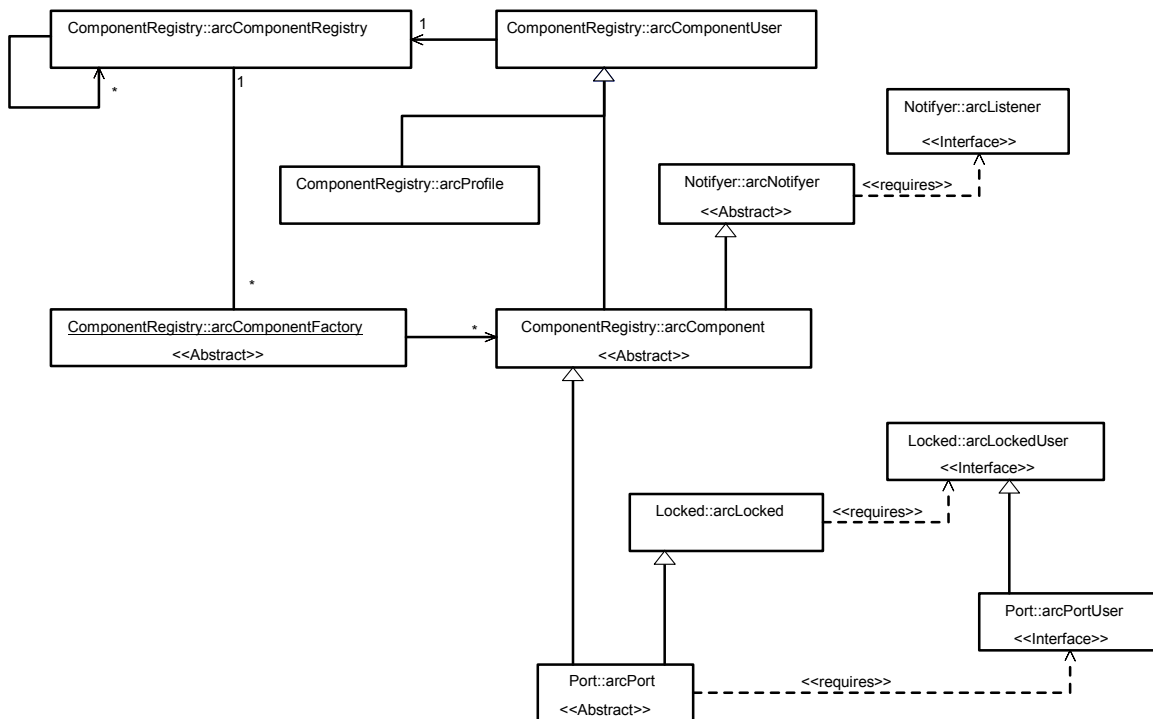
Fig. 6. Executable framework of the architecture
