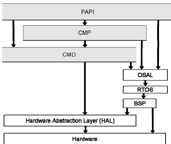
Fig. 5. The layers of the system
